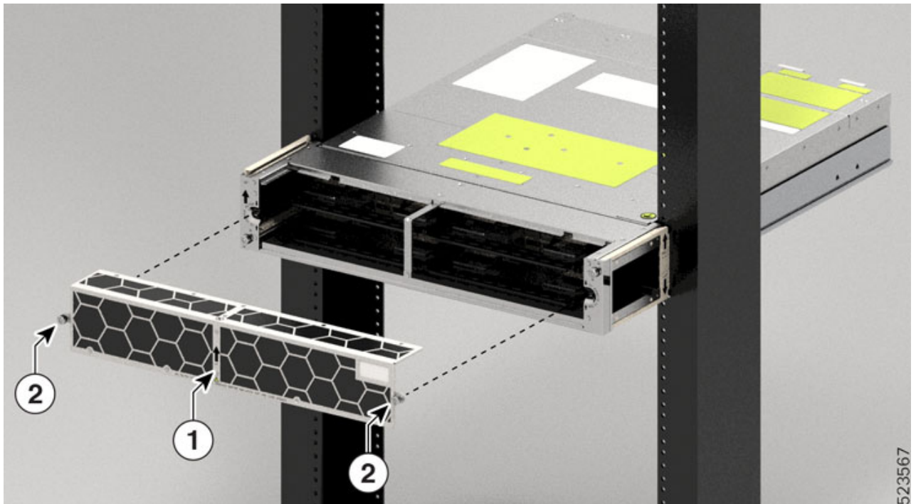
Figure 22: Installing the Air Filter
