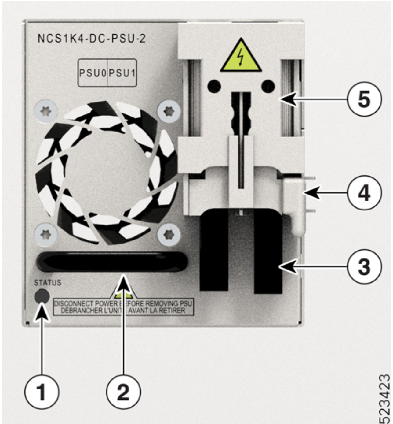
Figure 15: NCS1K4-DC-PSU-2 with 180-degree Power Lug Cable Connection
