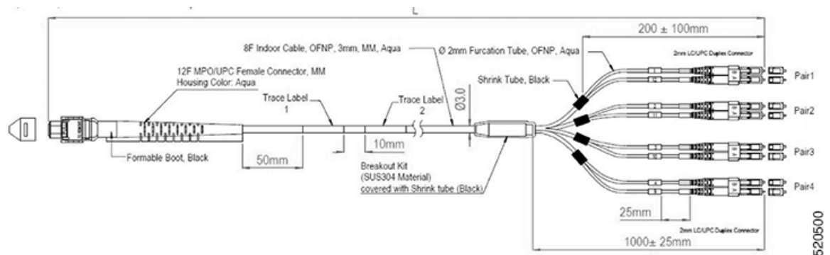
Figure 1: Breakout Cable
