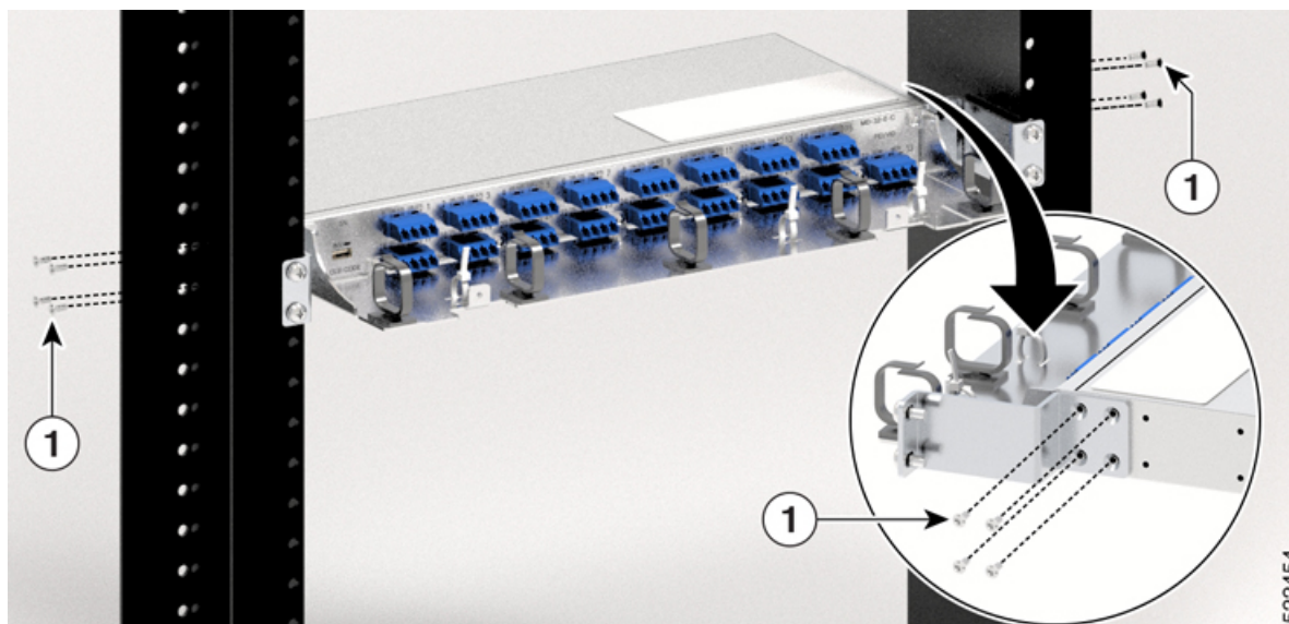
Figure 6: Mounting the Patch Panel on the ETSI Rack
