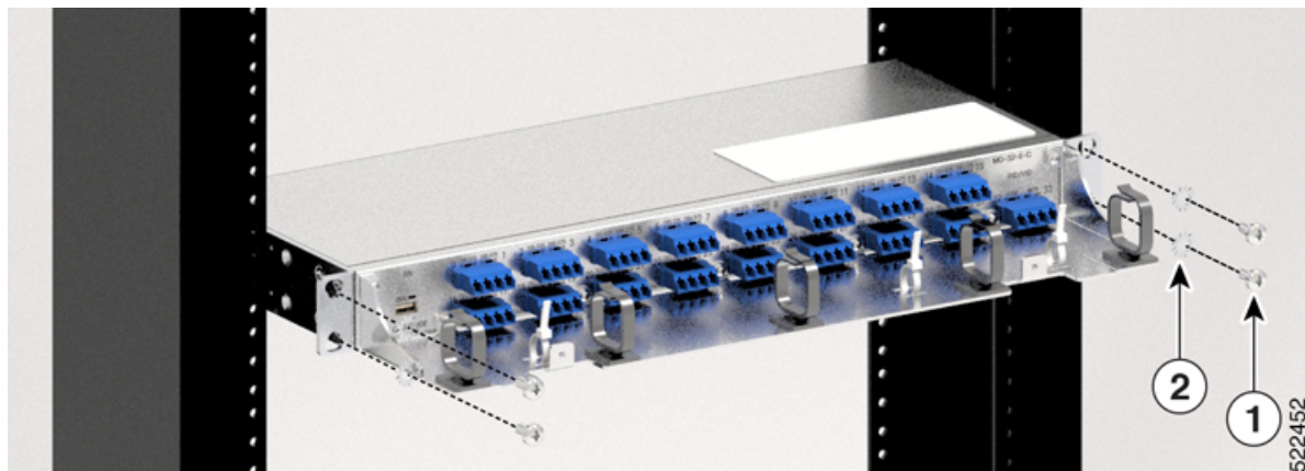
Figure 3: Installing the Adapter Bracket on a 19-inch Rack
