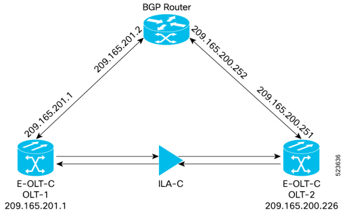
Figure 1: BGP Topology
