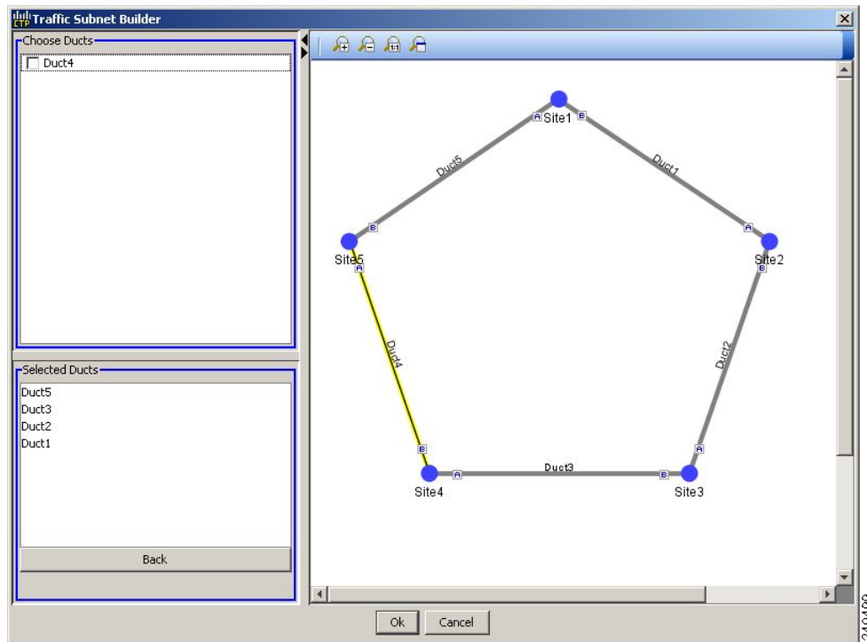
Figure 2-11 Traffic Subnet Builder Wizard
