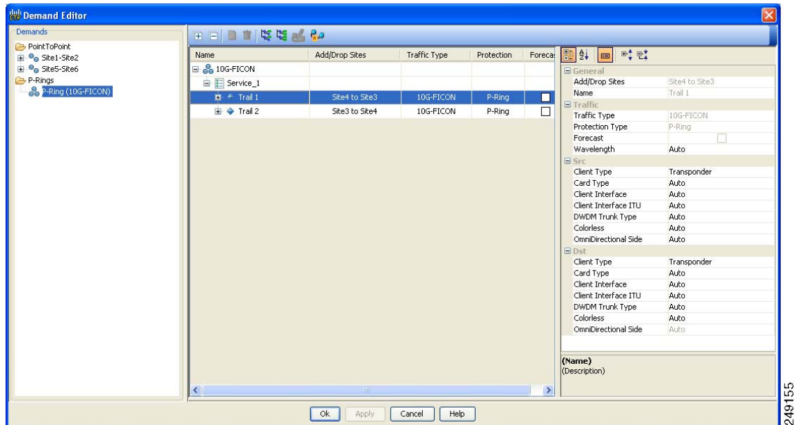
Figure 4-9 Edit P-Ring Demand Dialog Box
