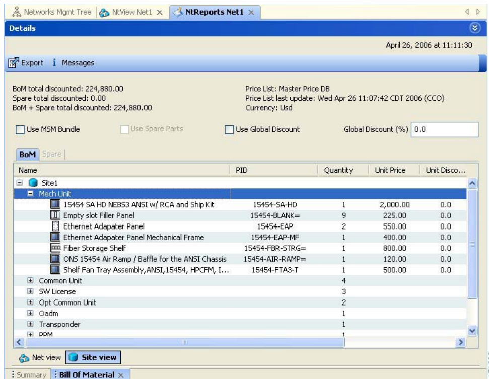
Figure 2-40 Bill of Material Tab, Site View Subtab
