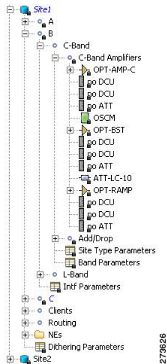
Figure 4-2 Analyzed Site in the Project Explorer
