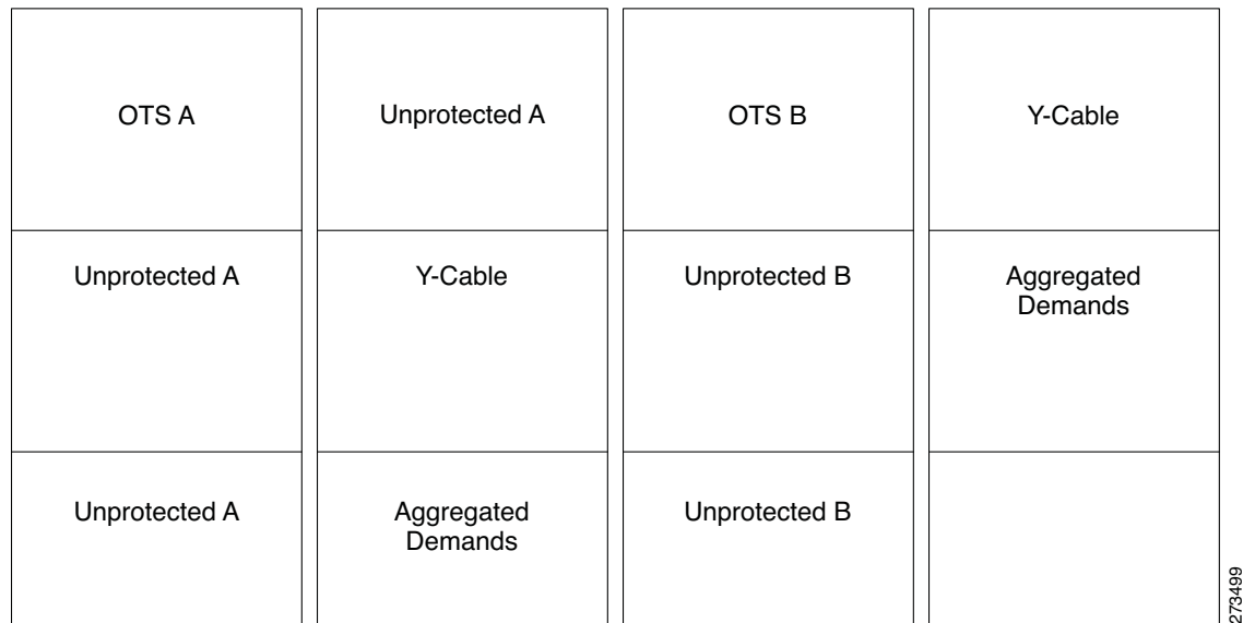
Figure 4-24 Client Shelf Placement-Protection and Aggregated Demand
