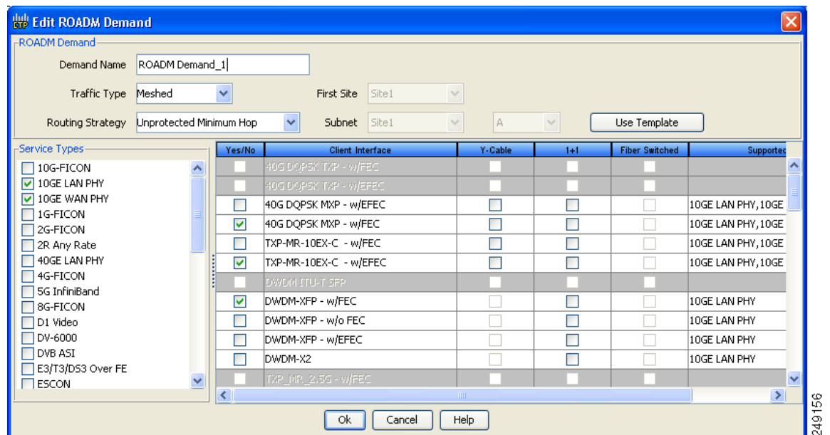
Figure 4-10 Edit ROADM Demand Dialog Box
