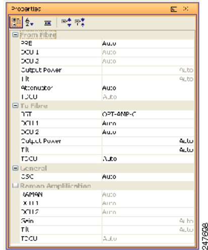
Figure 4-6 Properties Pane
