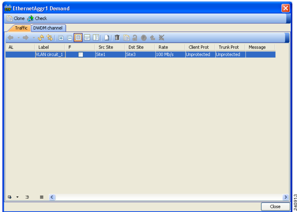
Figure 4-11 Ethernet Aggregated Demand Dialog Box
