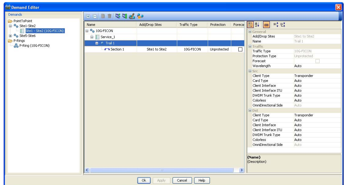
Figure 4-8 Edit Point-to-Point Demand Dialog Box
