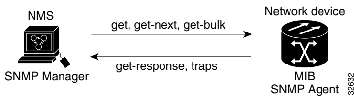
Figure 24-2 SNMP Network
