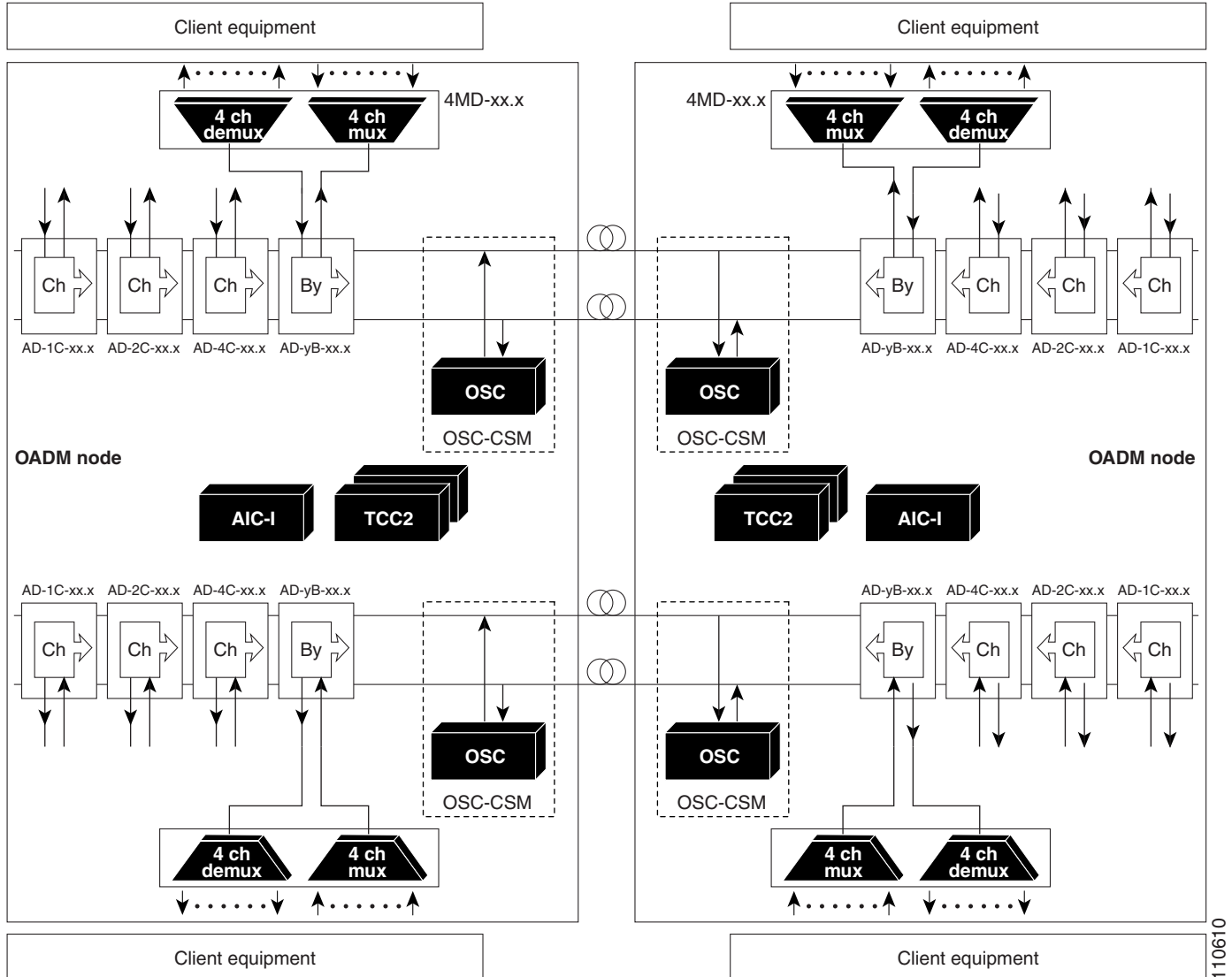
Figure 3-26 1+1 Protected Single-Span Link with Passive OADM Nodes
