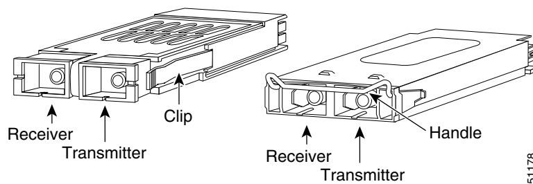
Figure 1-53 GBICs
