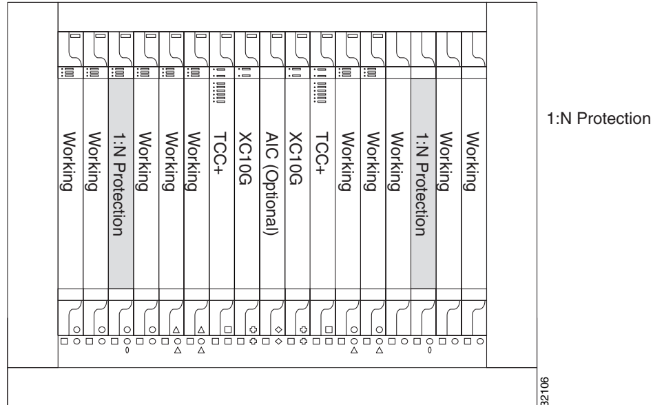
Figure 7-2 Example: ONS 15454 Cards in a 1:N Protection Configuration (SMB EIA)
