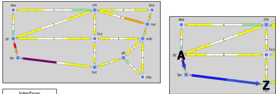
Figure 132: Network Before Optimization
