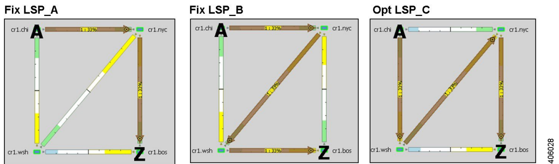
Figure 125: Example: Improved Global Optimization When Setting All LSPs to Opt
