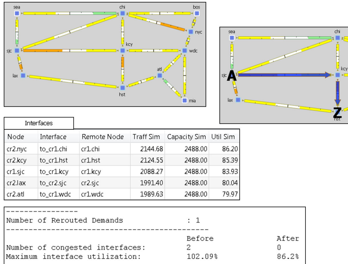
Figure 133: Network After Reducing Utilization to Below 90%
