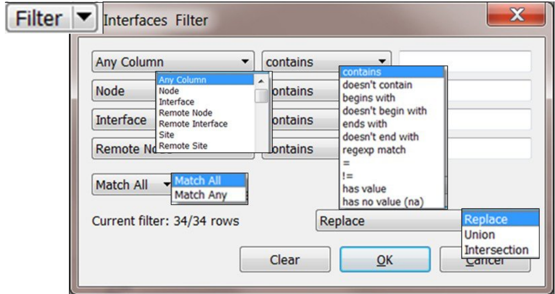
Figure 7: Interfaces Filter
