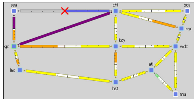
Figure 134: Optimized Network Under Failure
