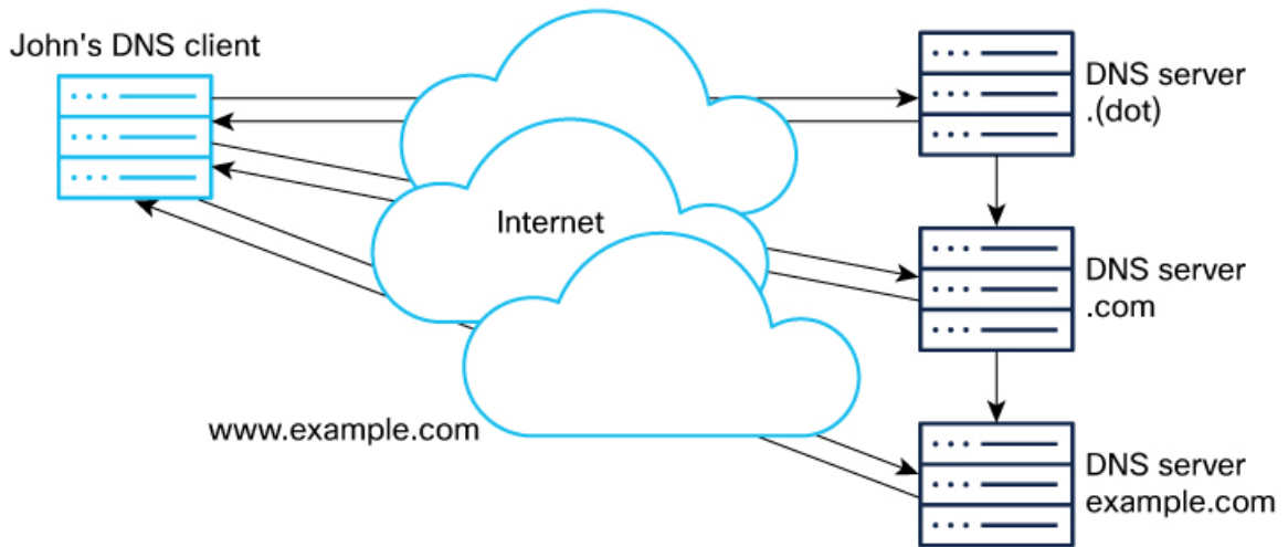
Figure 3: DNS Hierarchical Name Search
