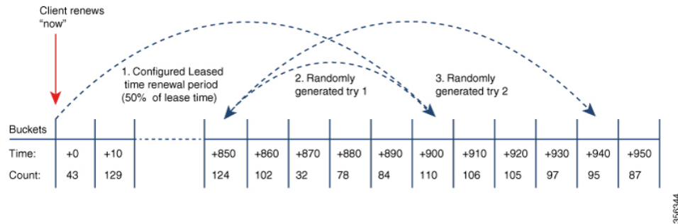
Figure 14: Distribute Lease Renewals Example
