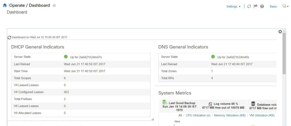
Figure 17: Preset Dashboard Elements
