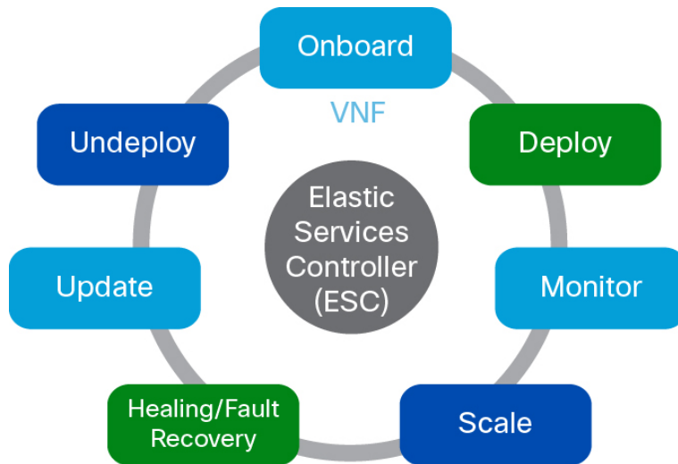
Figure 2: ESC Lifecycle
