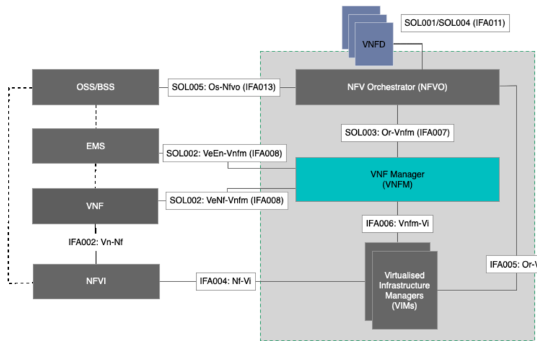
Figure 1: NFV MANO Architecture with Reference Points
