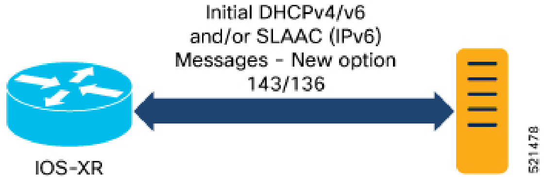
Figure 3: DHCP discovery
