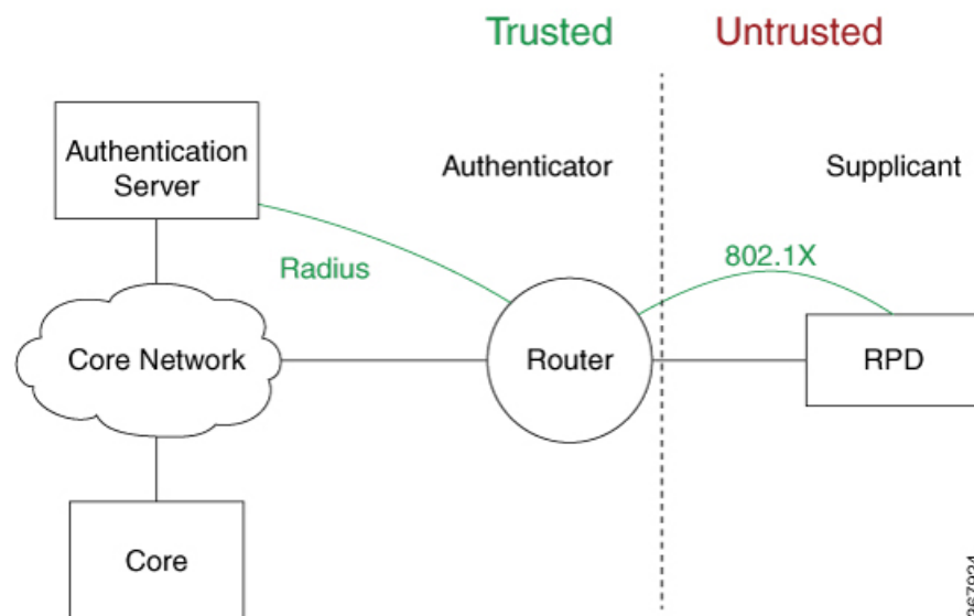
Figure 4: Topology for IEEE 802.1X Port-Based Authentication
