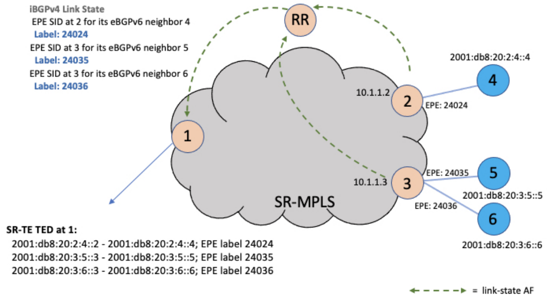
Figure 6: BGP-LS
