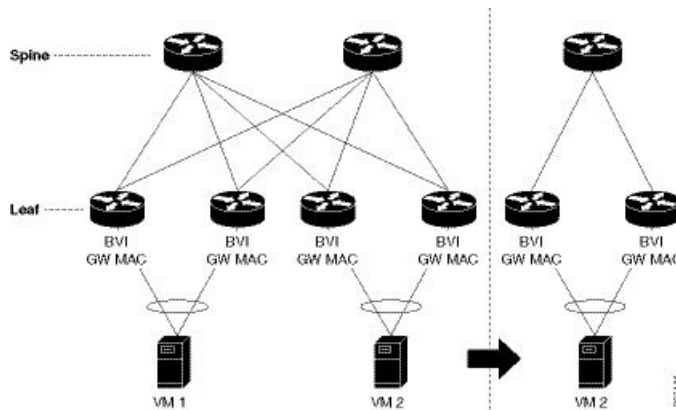
Figure 58: EVPN IRB
