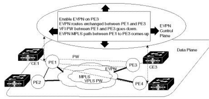
Figure 45: EVPN MPLS Seamless Integration with VPLS
