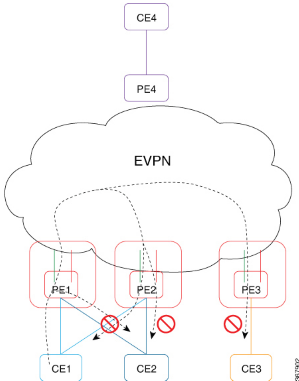
Figure 62: EVPN E-Tree
