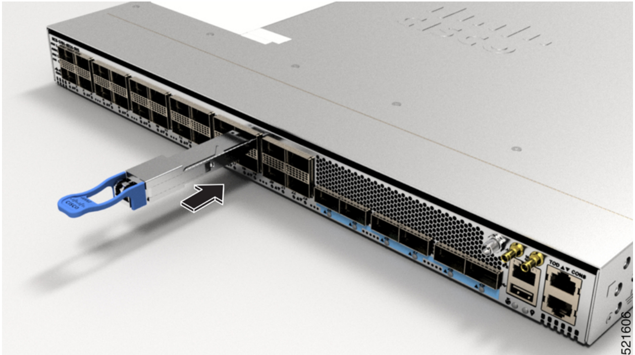
Figure 9: Inserting QSFP-DD Transceiver Module
