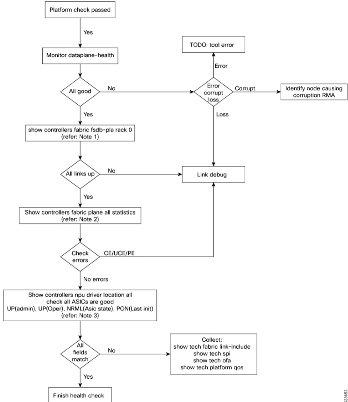
Figure 10: Troubleshooting Flowchart
