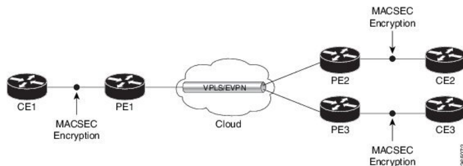
Figure 11: MACSec in a VPLS/EVPN Cloud
