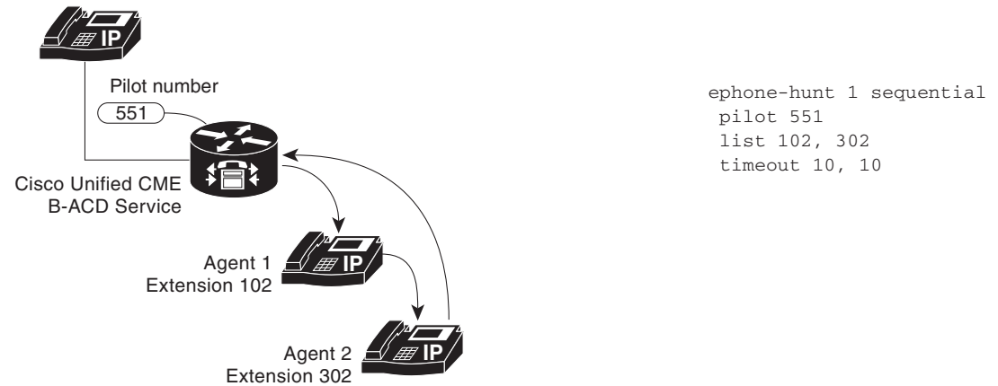
Figure 4-2 B-ACD Hunt Group Example
