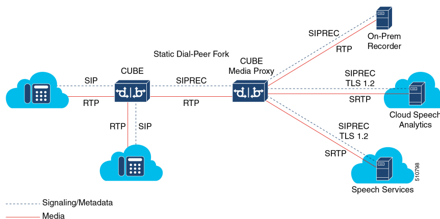
Figure 44: Deployment Scenario for SIPREC-Based CUBE Media Proxy
