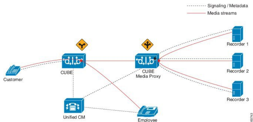
Figure 42: Deployment Scenario for CUBE Media Proxy Using Unified CM NBR for External Call
