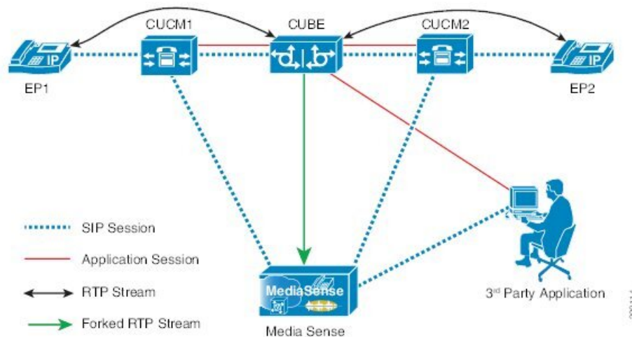
Figure 45: Forking Preservation
