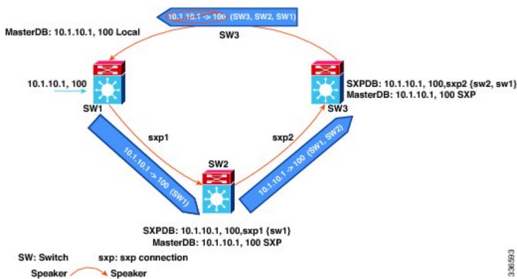
Figure 3: SXPv4 Loop Detection
