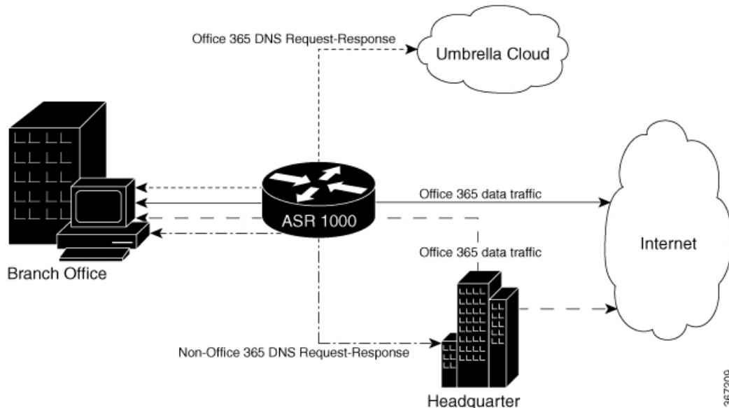
Figure 3: DCA for Office 365
