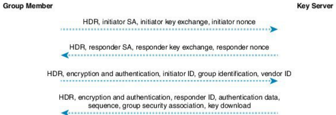
Figure 16: G-IKEv2 Message Exchanges
