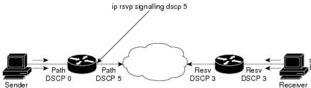
Figure 7: Control Plane DSCP Support for RSVP
