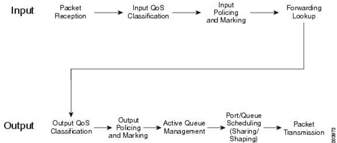
Figure 4: QoS Packet Processing
