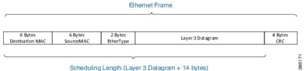
Figure 6: Scheduling Length
