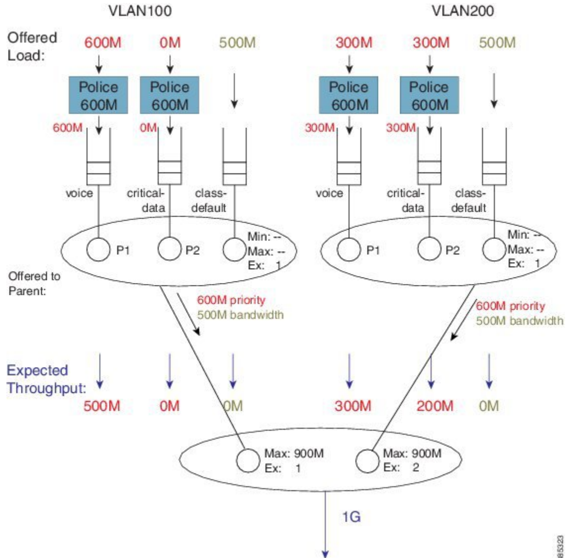
Figure 14: Child Schedule Apportions Bandwidth received from Parent Schedule
