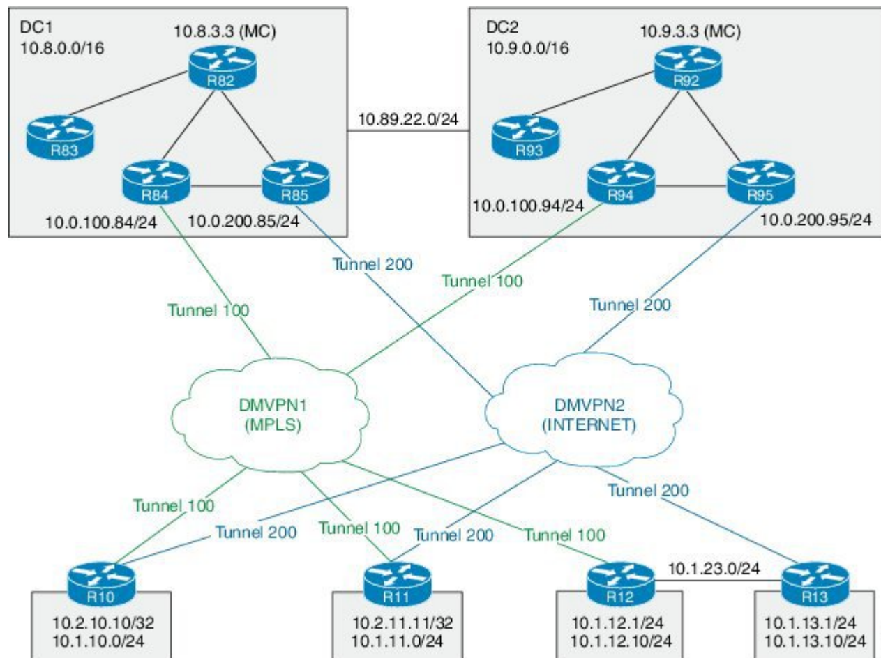
Figure 7: PfRv3 Transit Hub Topology
