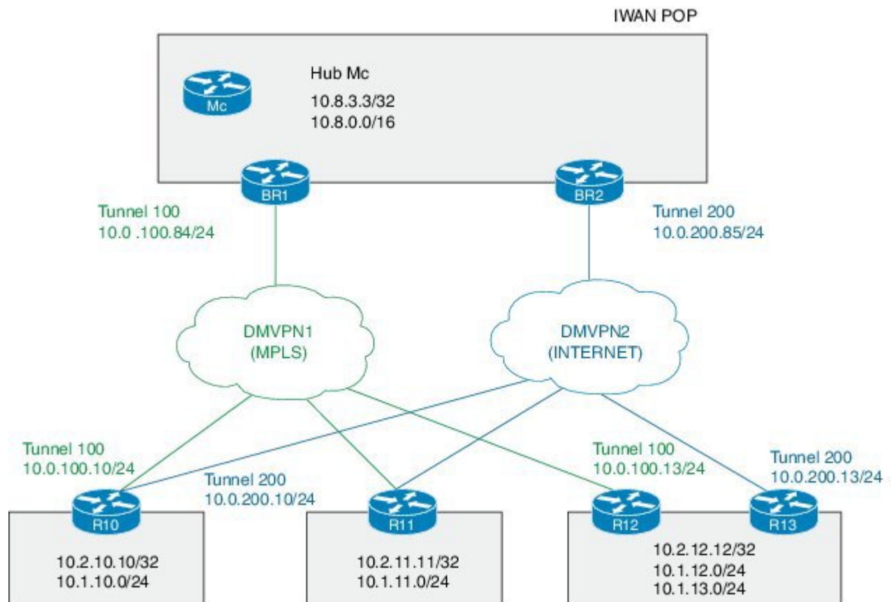
Figure 9: PfRv3 Topology
