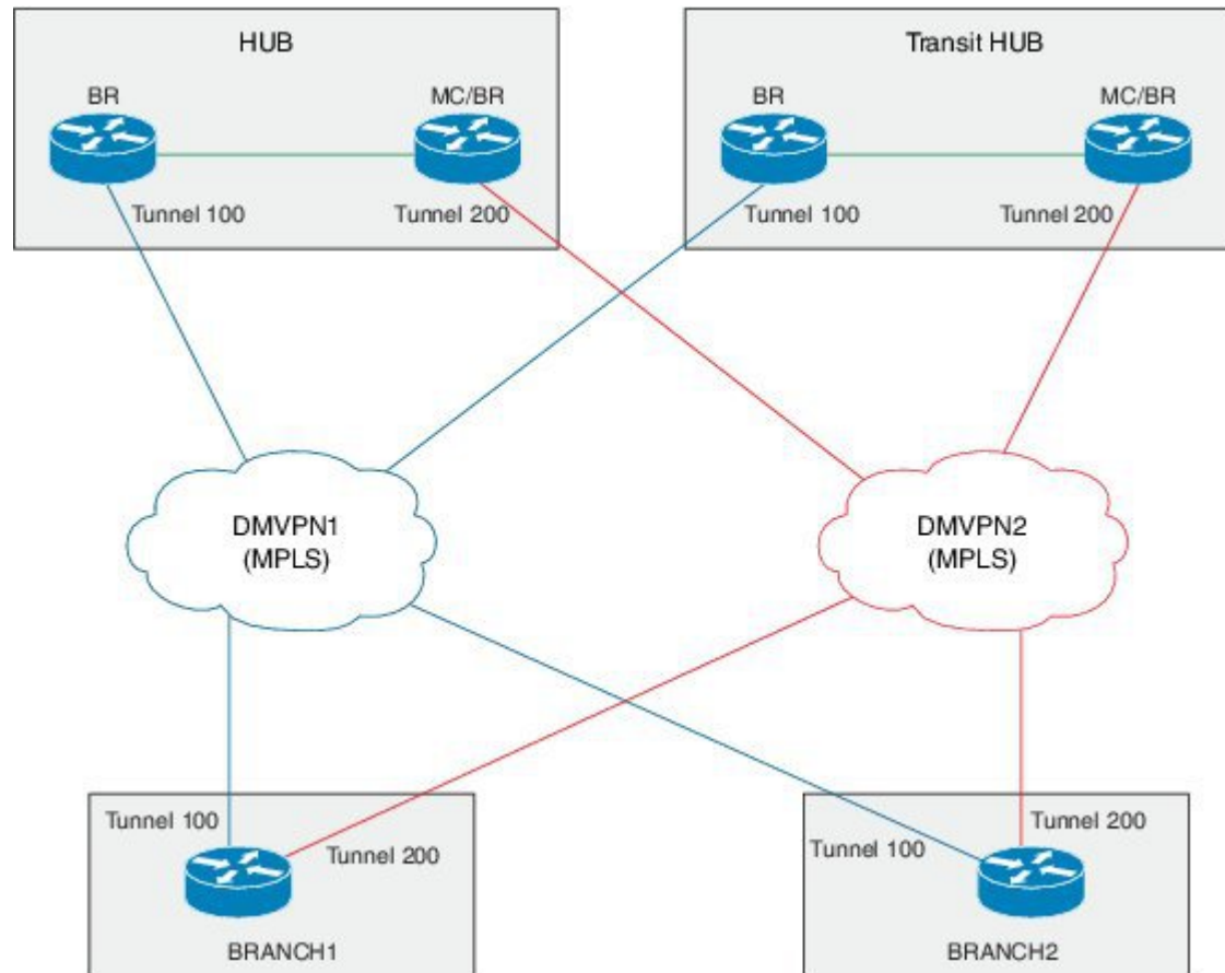
Figure 5: Dual Data Center with Multiple Borders
