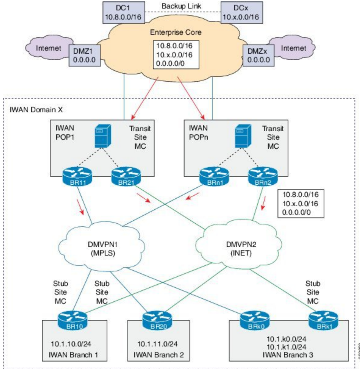
Figure 6: Dual Data Center with Same Prefix
