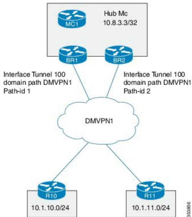
Figure 4: Single Data Center with Multiple Borders
