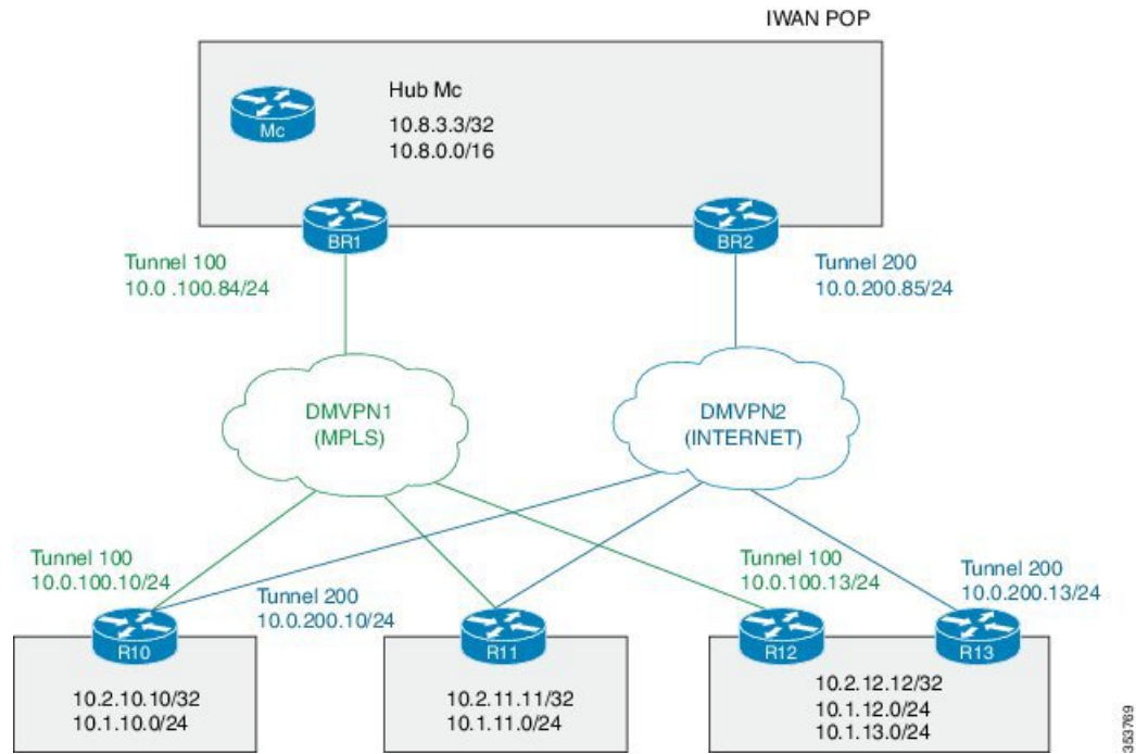
Figure 2: PfRv3 Topology
