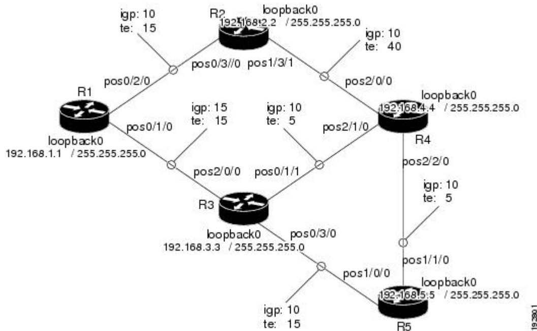
Figure 4: Network Topology
