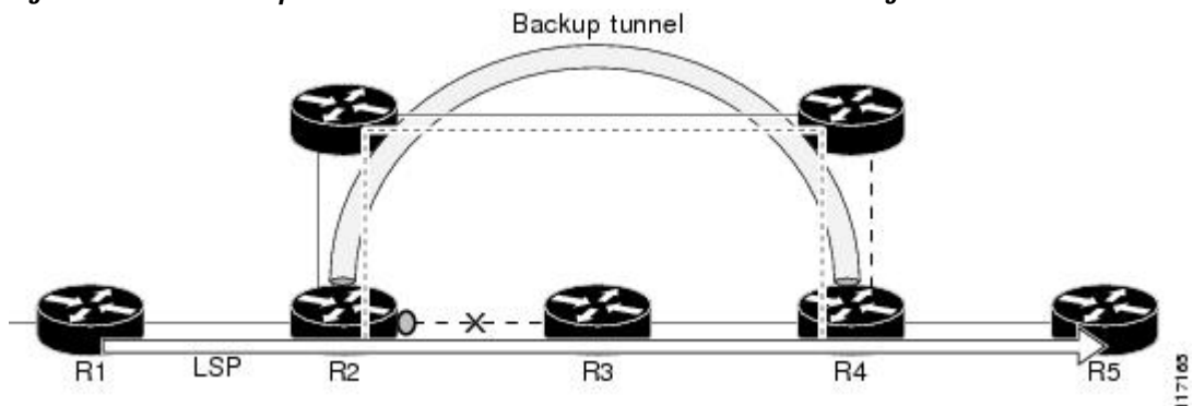
Figure 18 Backup Tunnel in the Same SRLG as the Interface It Is Protecting
