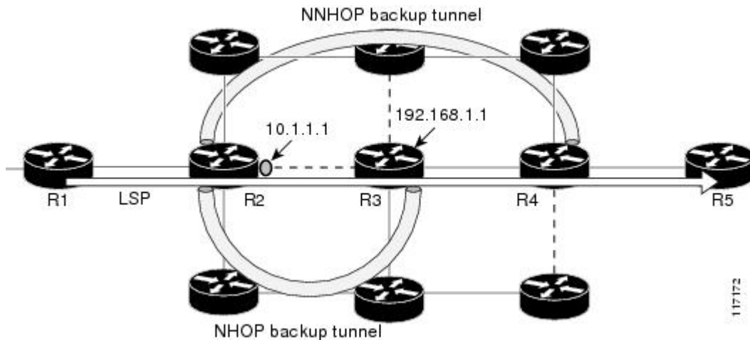
Figure 21 NNHOP Backup Tunnel
