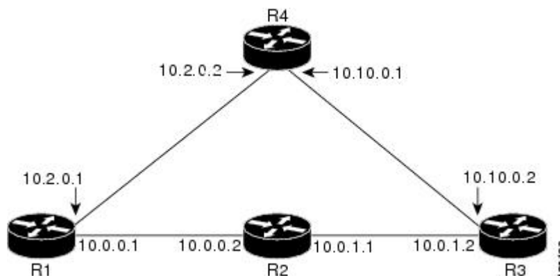
Figure 8 Network Topology--Path Protection
