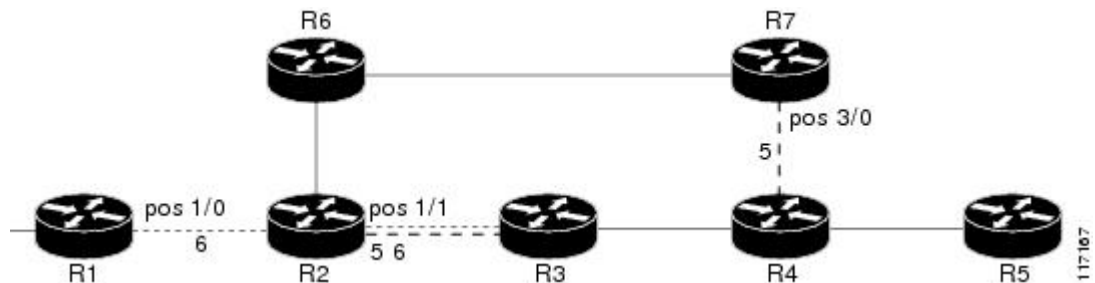
Figure 24 SRLG Membership
