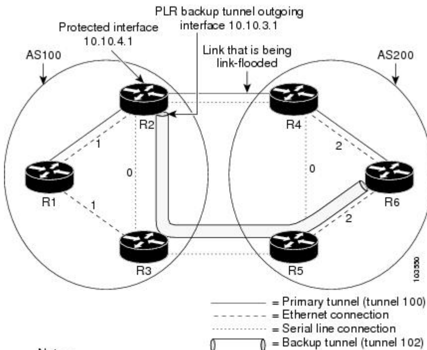
Figure 27 ASBR Node Protection
