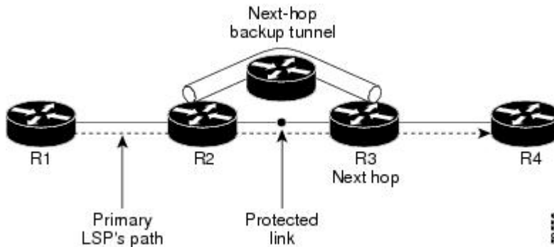
Figure 15 Next-Hop Backup Tunnel
