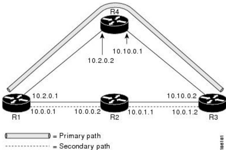
Figure 9 Network Topology Verification
