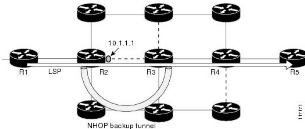
Figure 26 srlg exclude force--NHOP Autobackup Tunnel
