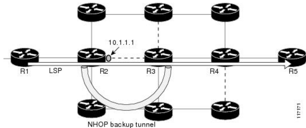
Figure 23 Autotunnel Backup for NHOP
