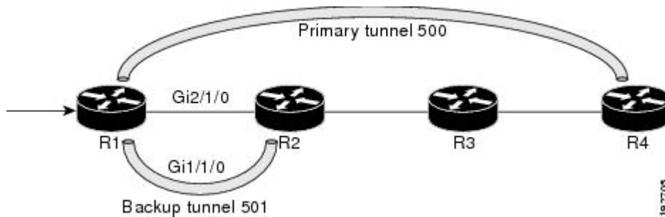
Figure 13 Protected LSPs
