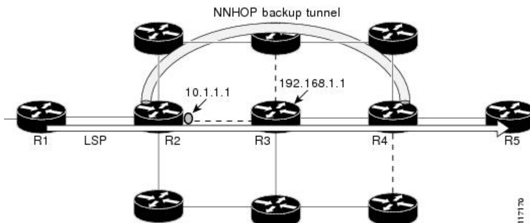
Figure 25 srlg exclude force--NNHOP Autobackup Tunnel
