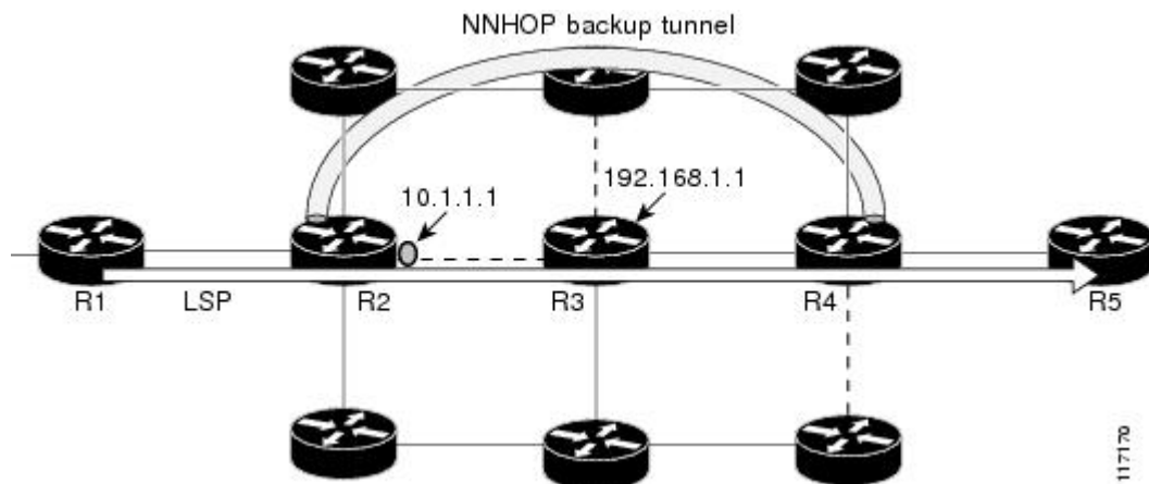
Figure 23 srlg exclude force--NNHOP Autobackup Tunnel
