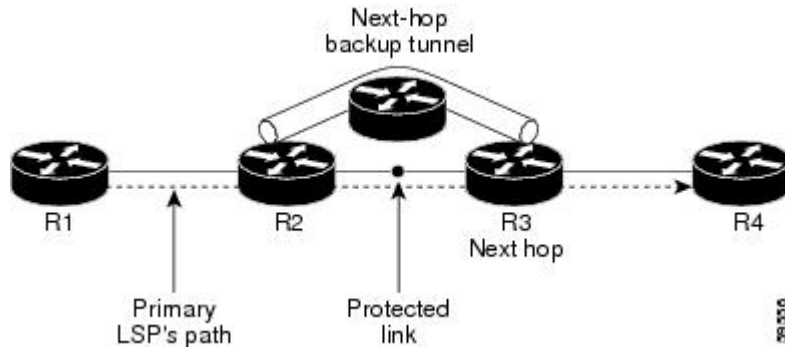
Figure 13 Next-Hop Backup Tunnel
