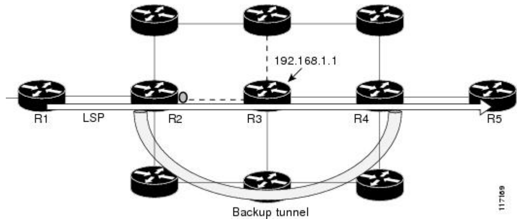
Figure 20 Autotunnel Backup for NNHOP
