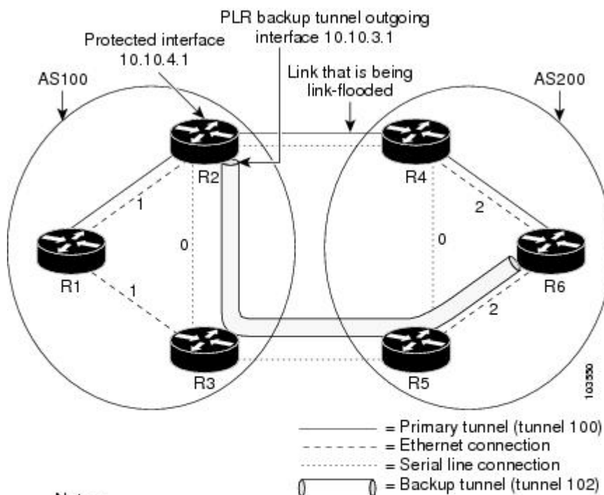
Figure 25 ASBR Node Protection
