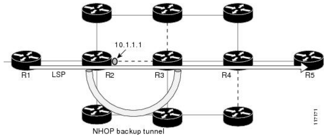
Figure 21 Autotunnel Backup for NHOP
