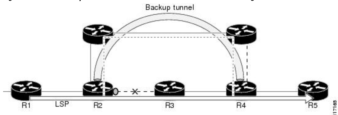
Figure 16 Backup Tunnel in the Same SRLG as the Interface It Is Protecting
