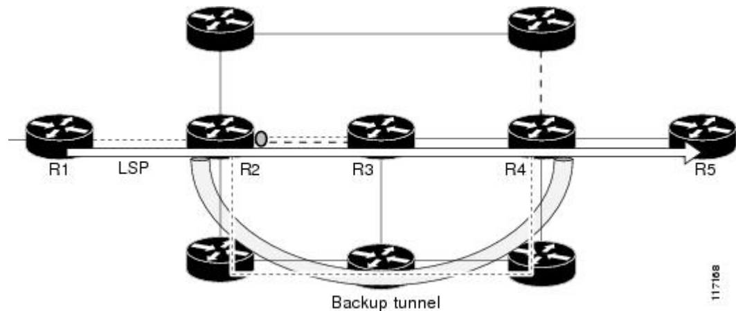
Figure 17 Backup Tunnel That Avoids SRLG of Protected Interface
