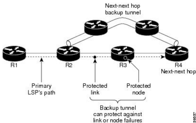
Figure 14 Next-Next Hop Backup Tunnel
