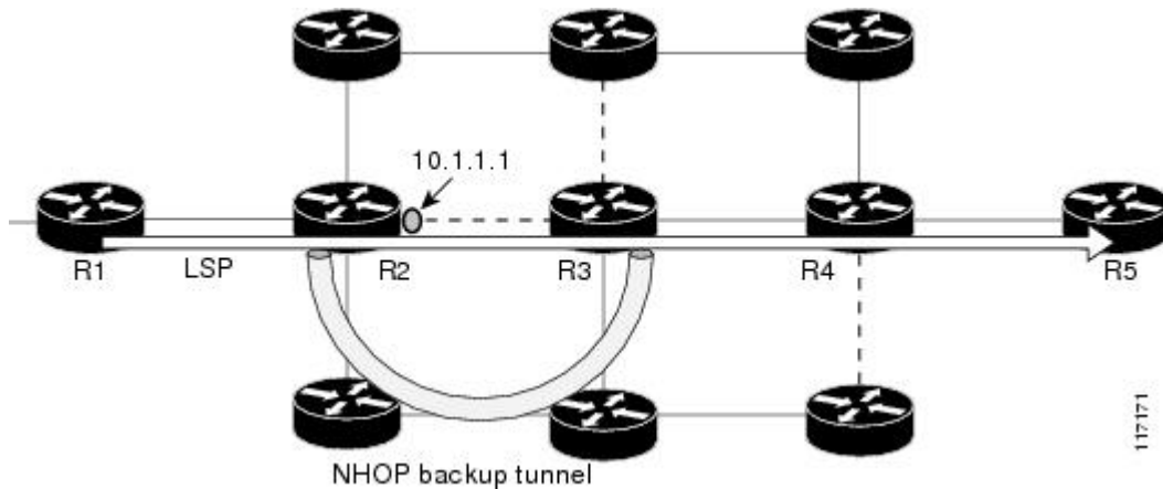
Figure 18 NHOP Backup Tunnel
