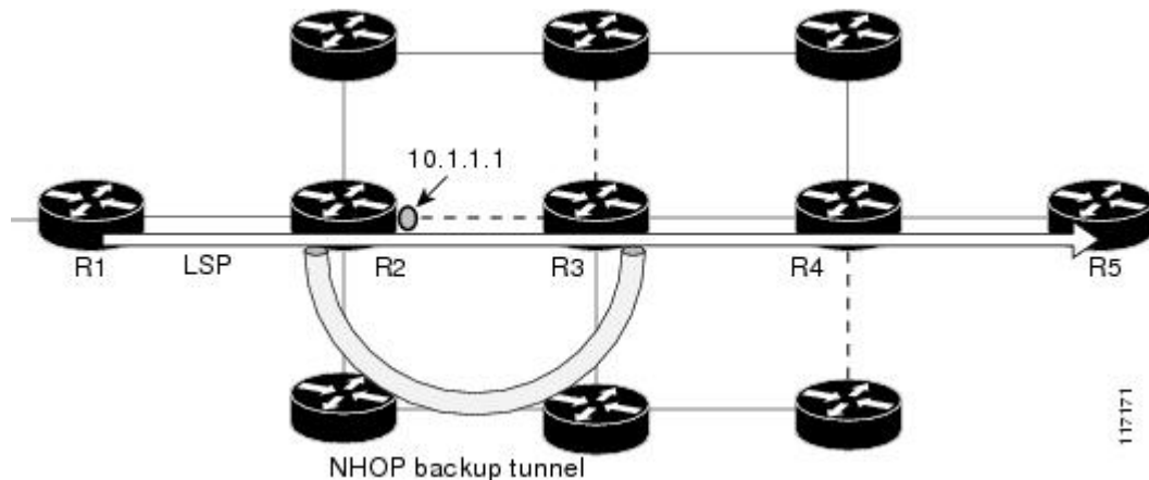
Figure 24 srlg exclude force--NHOP Autobackup Tunnel
