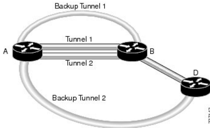
Figure 15 Specifying Link Attributes and Affinity with Autotunnel Backup
