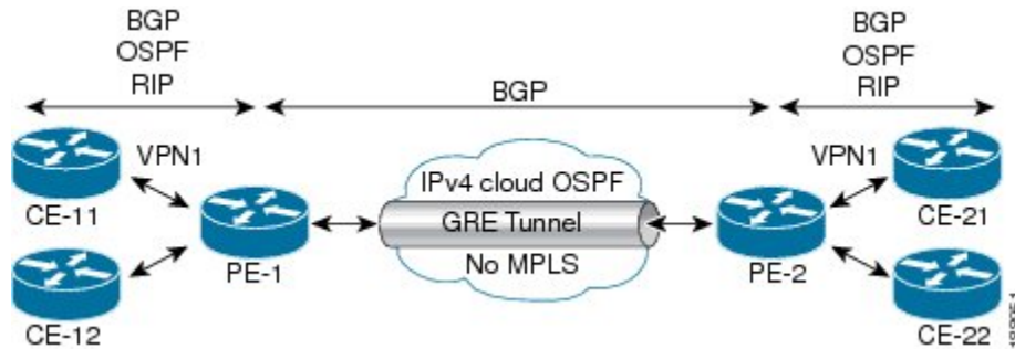
Figure 1: PE-to-PE Tunneling
