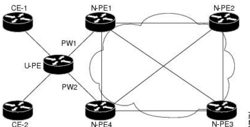
Figure 13 H-VPLS N-PE Redundancy for QinQ and MPLS Access with MPLS Access Based on Pseudowire Redundancy
