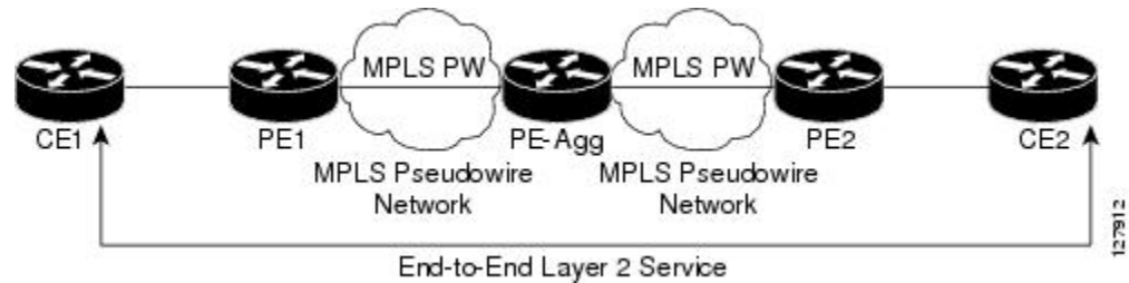
Figure 10 L2VPN Pseudowire Switching in an Inter-AS Topology
