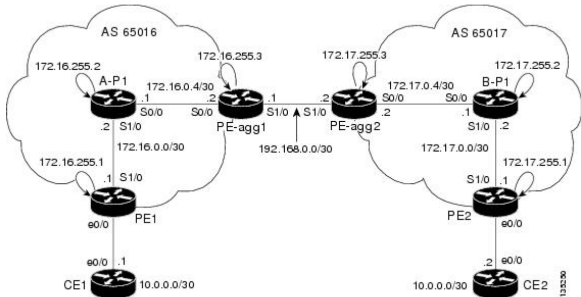
Figure 11 L2VPN Pseudowire Switching in an Interautonomous System
