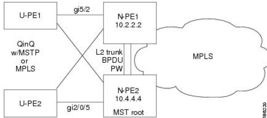
Figure 14 H-VPLS N-PE Redundancy with QinQ Access Topology
