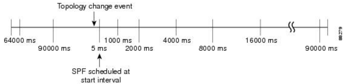
Figure 14: Timer Intervals Reset after Topology Change Event
