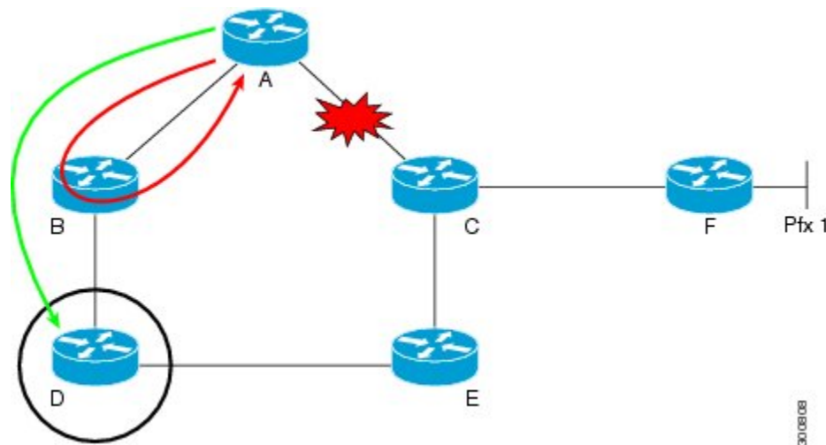
Figure 13: Remote LFA IPFRR with Ring Topology
