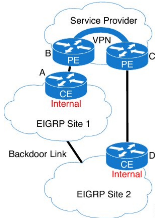
Figure 1: EIGRP 6PE/6VPE Functionality
