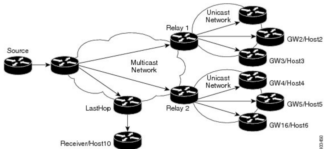
Figure 15: Automatic Multicast Tunneling (AMT)
