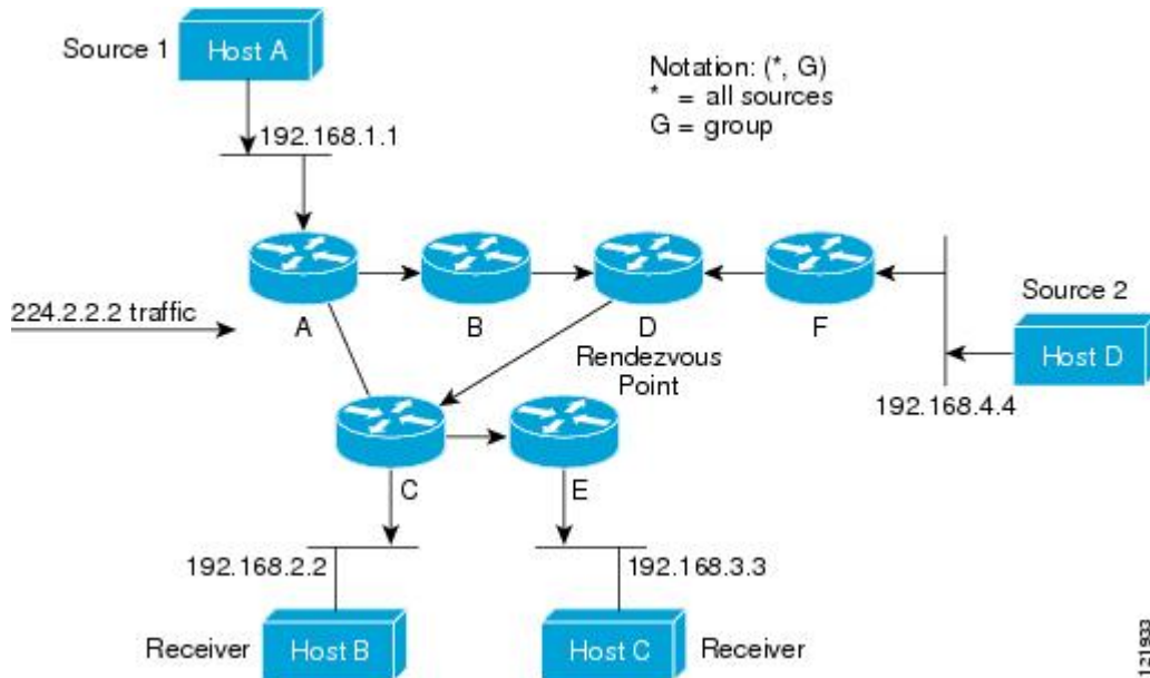
Figure 1: Shared Tree
