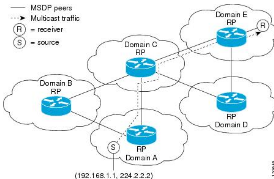
Figure 7 MSDP Sharing Source Information Between RPs in Each Domain
