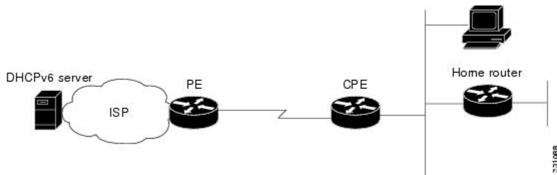
Figure 2: Broadband Topology
