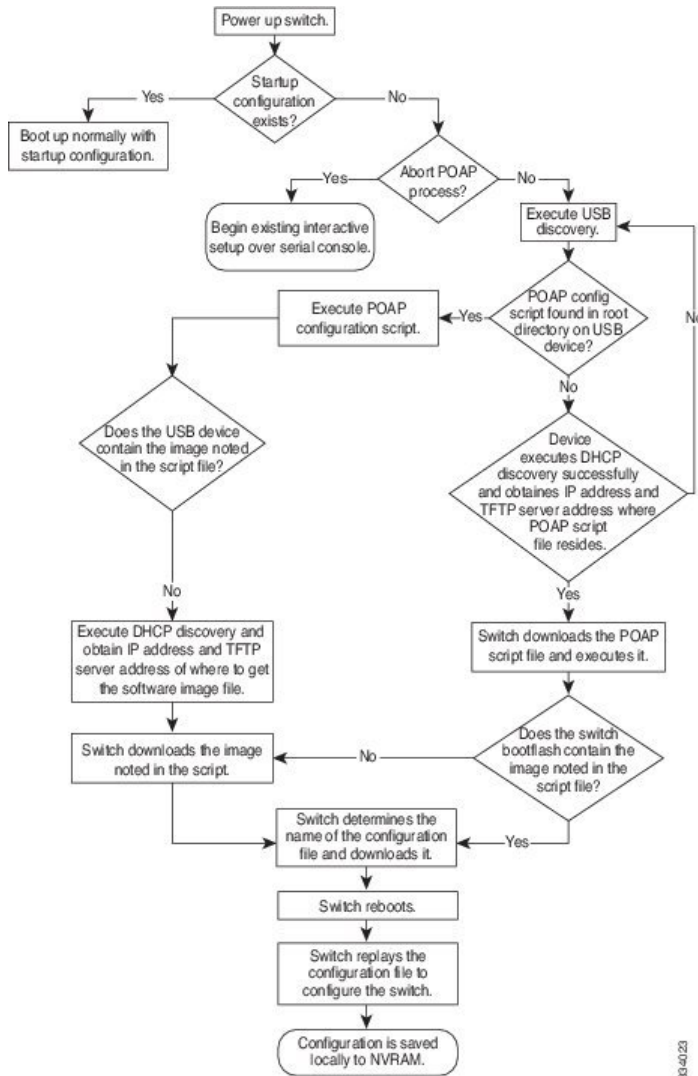
Figure 4: POAP Process
