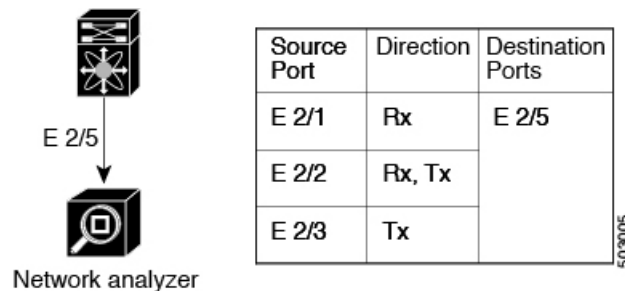
Figure 7: SPAN Configuration
