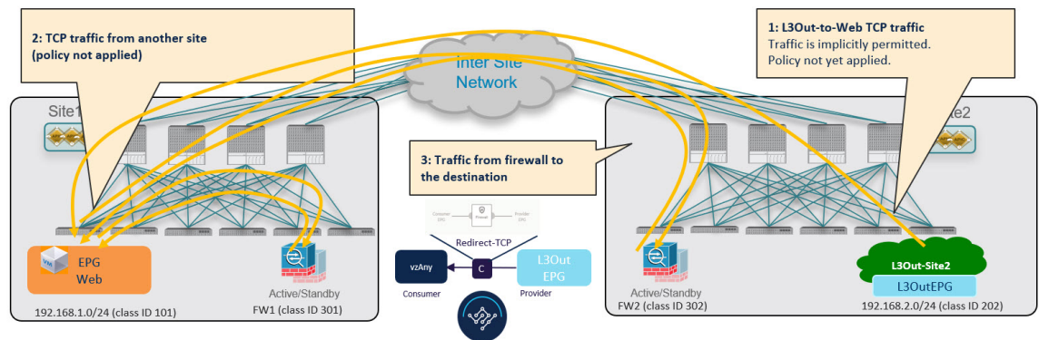
Figure 10: vzAny-to-L3Out Provider-to-Consumer Traffic Flow (Initial Traffic and Conversational Learning)
