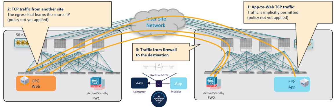
Figure 7: vzAny-to-EPG Provider-to-Consumer Traffic Flow (Initial Traffic and Conversational Learning)
