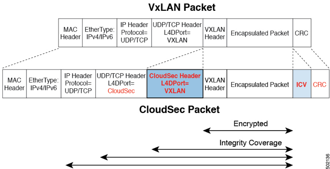
Figure 12: CloudSec Packet
