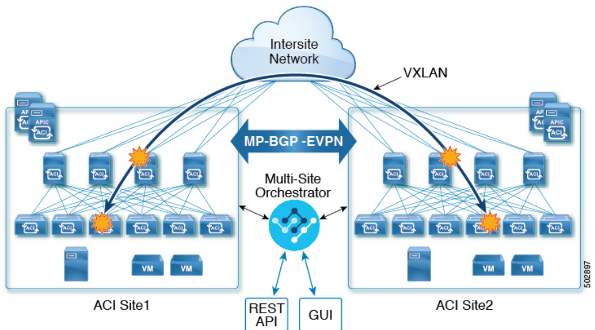
Figure 33: Multi-Site and ISN
