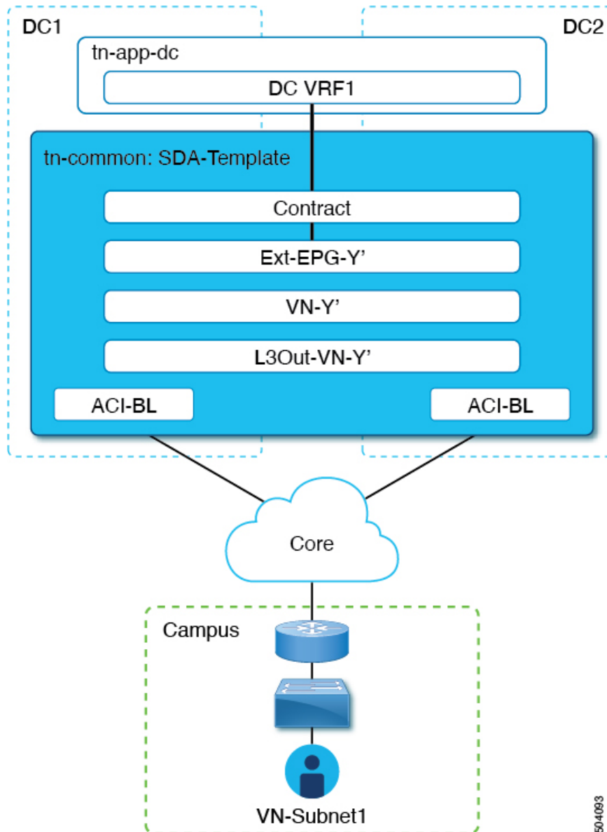
Figure 26: Mapping to a VRF
