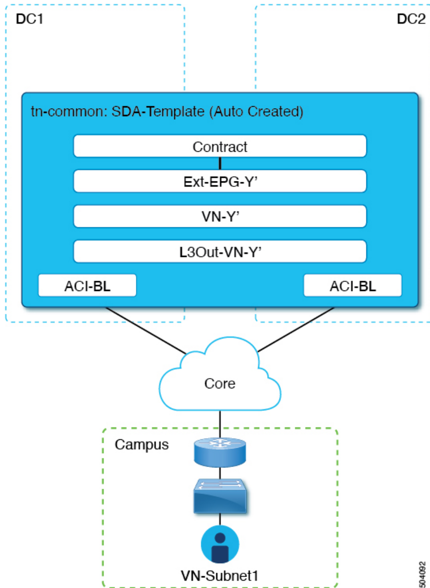
Figure 25: Extending a VN
