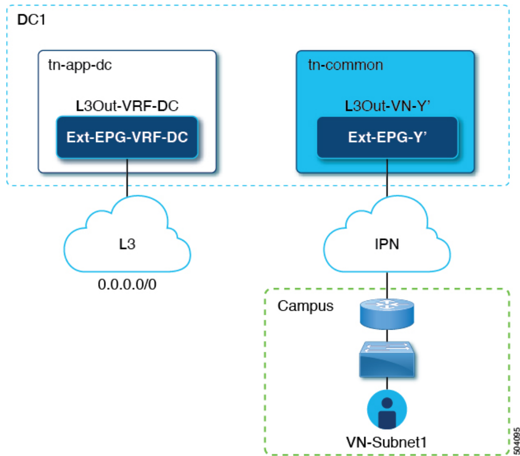
Figure 28: L3Out connection
