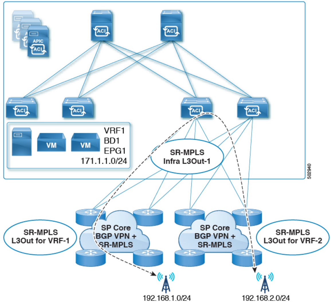
Figure 36: Transit Routing Configuration Using Different VRFs
