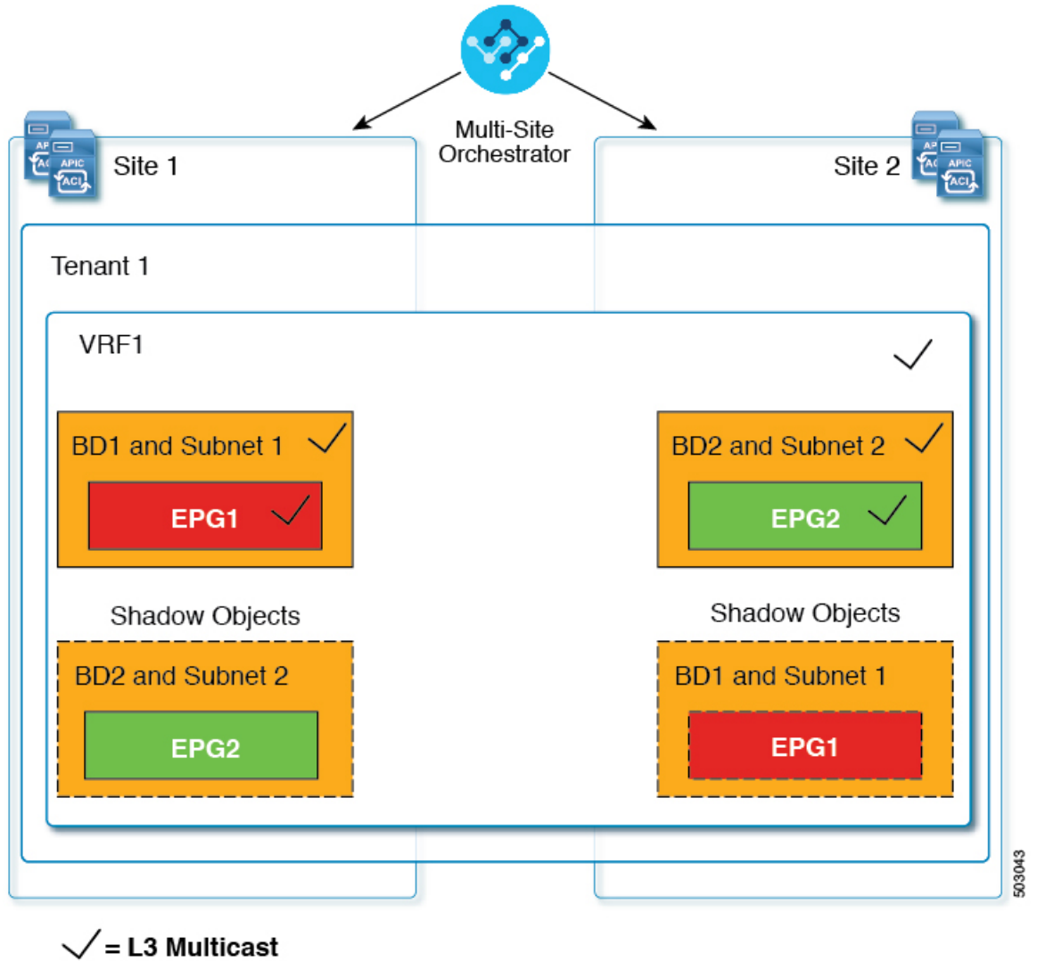
Figure 5: L3 Multicast
