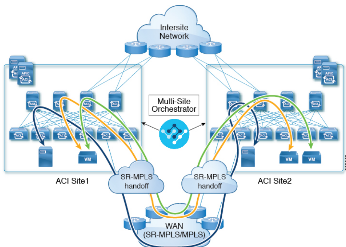
Figure 34: Multi-Site and MPLS
